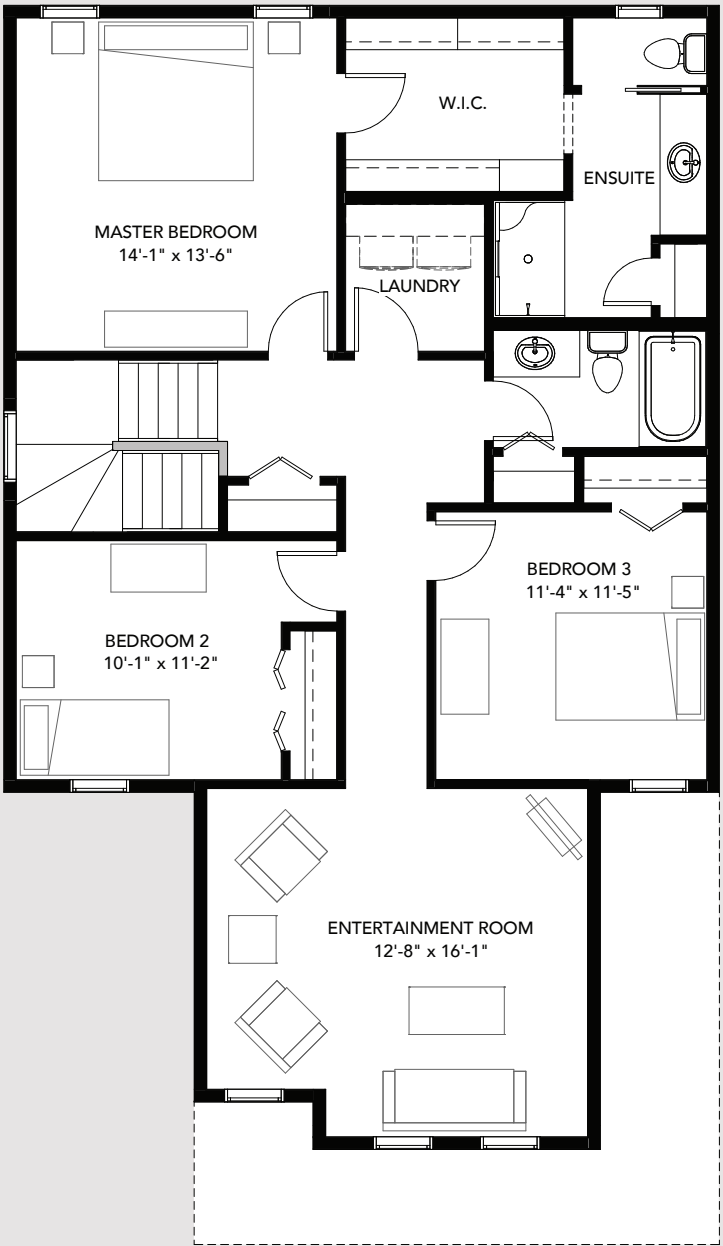
UPPER FLOOR 1235 sq. ft.
