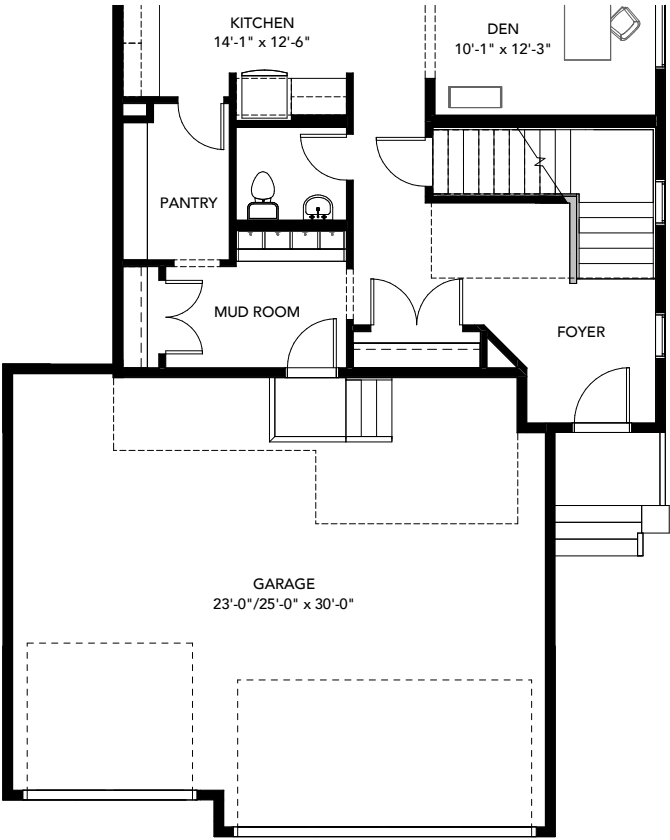
MAIN FLOOR 3 CAR OPTION 1224 sq. ft.
