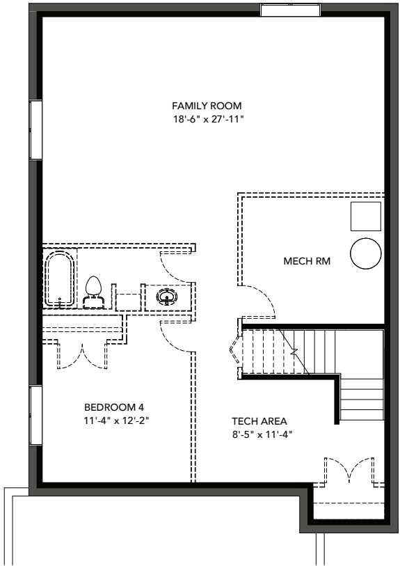
LOWER FLOOR FUTURE DEVELOPMENT 872 sq. ft.
