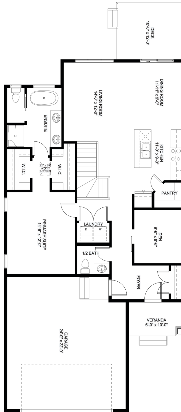
MAIN FLOOR PLAN 1248 sq. ft.
