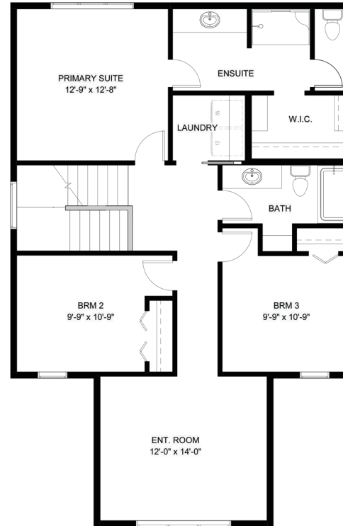
UPPER FLOOR 1101 sq. ft.
