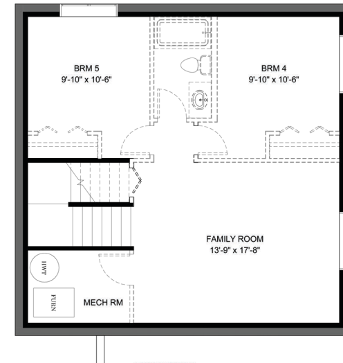
LOWER FLOOR FUTURE DEVELOPMENT 572 sq. ft.
