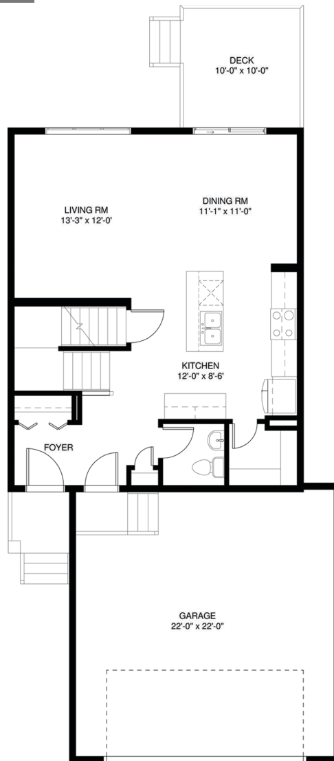
MAIN FLOOR 708 sq.ft.
