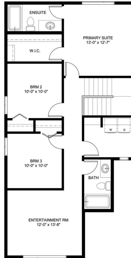
UPPER FLOOR 1011 sq.ft.
