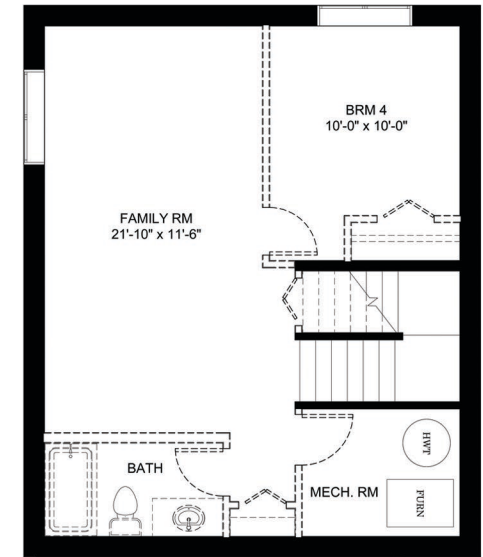
LOWER FLOOR FUTURE DEVELOPMENT 458 sq.ft.
